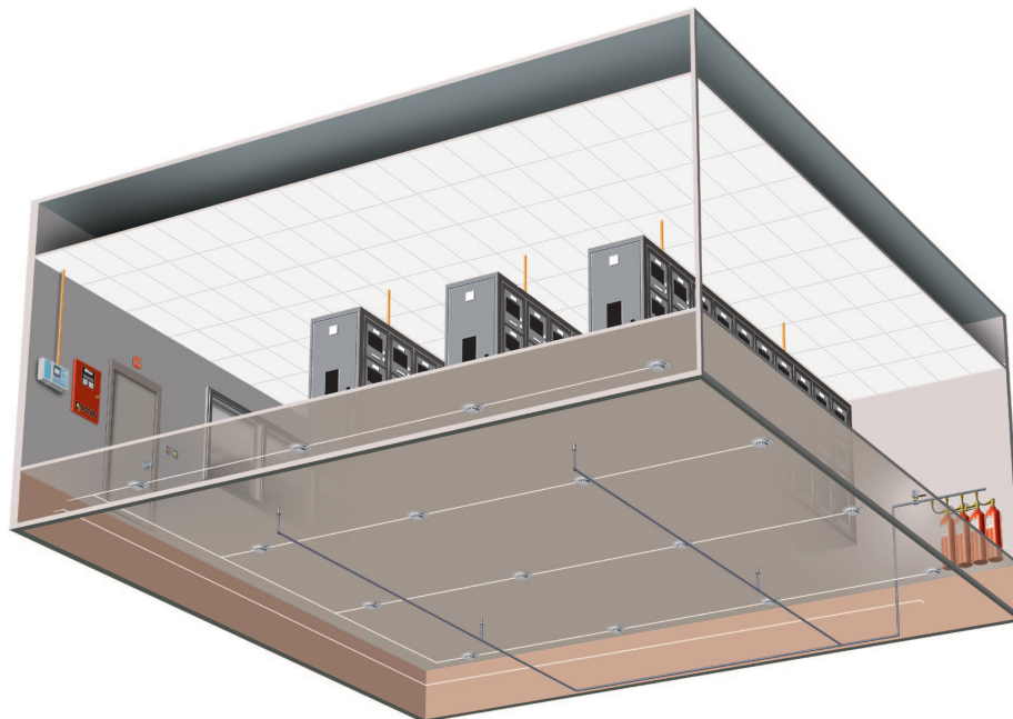
“Space Beneath a Raised Floor” protect by a Fike Carbon Dioxide Extinguishing System
